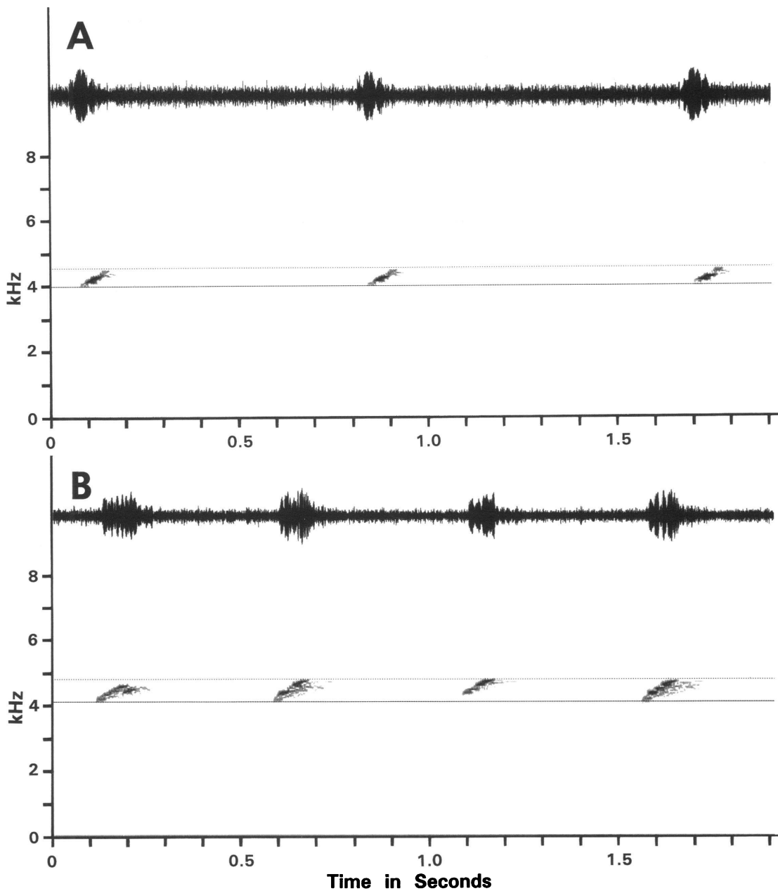
Fig. 6. Advertisement calls of two individuals of Epipedobates simulans from ridge along Río Távora (vicinity of type locality), Depto. Puno, shown as narrow-band (59 Hz) spectrograms, with matching waveforms. A. From 550 m elevation. Frequency cursors set at 4000 and 4560 Hz. B. A faster call from a site below 500 m elevation. Frequency cursors at 4120 and 4800 Hz. Both recorded by L. O. Rodríguez, June 3, 1992, temperatures not noted (AMNH herpetology reel 268).
